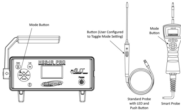
Figure 1 Toggling Between Search and Measure Modes
