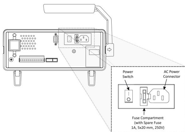
Figure 24 Location of Fuse Holder
