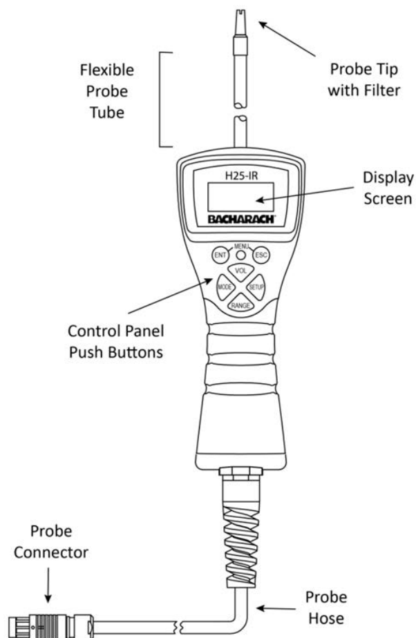
Figure 8 Components of the Smart Probe
