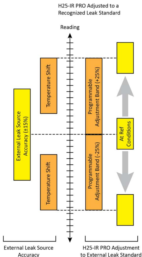
Figure 3 Adjusting the H25-IR Pro to a Recognized Leak Standard
