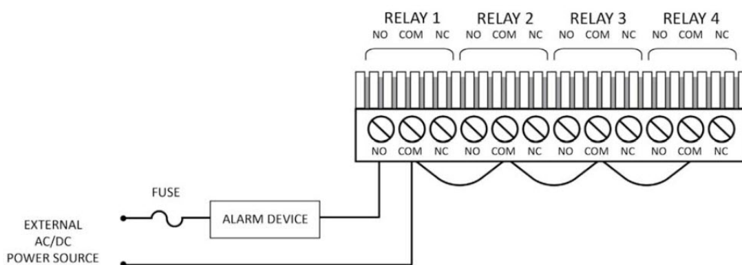
Figure 16 Sample Relay Wiring
