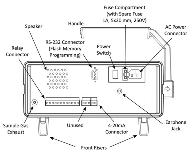
Figure 5 Back Panel Components of the H25-IR PRO
