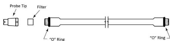
Figure 25 Probe Filter and "O" Ring Locations
