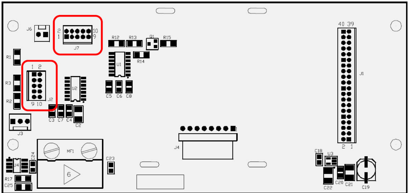
Figure 17 Front Panel Printed Circuit Board Containing Probe Connectors J2 and J7
