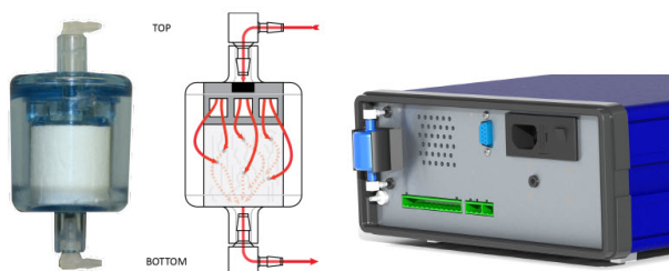
Figure 26 Back Panel of the H25-IR Pro showing Proper Orientation of the External Filter
