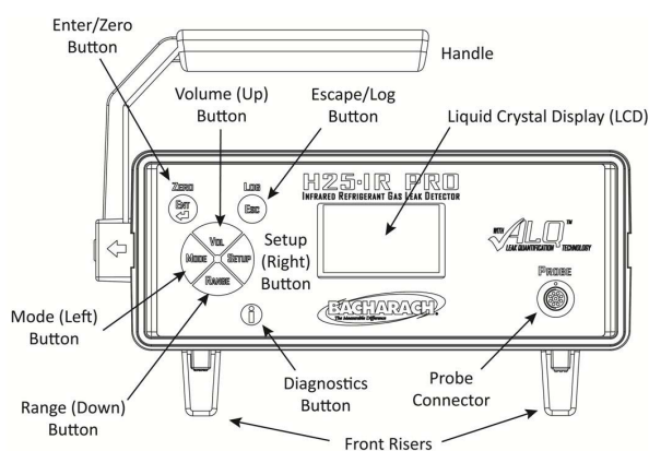
Figure 4 Front Panel Components of the H25-IR PRO
