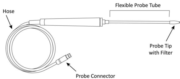
Figure 6 Components of the Standard Probe with Flexible Tubing
