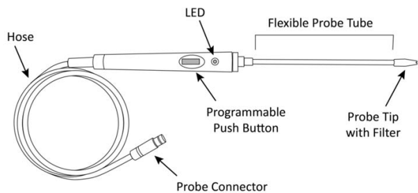
Figure 7 Components of the Standard Probe with LED and Push Button
